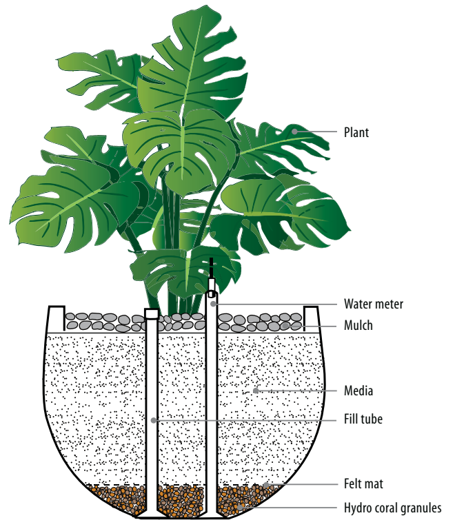
Self-watering system
