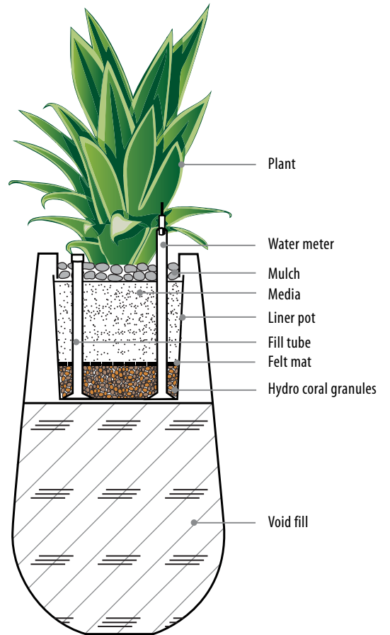
Self-watering system
