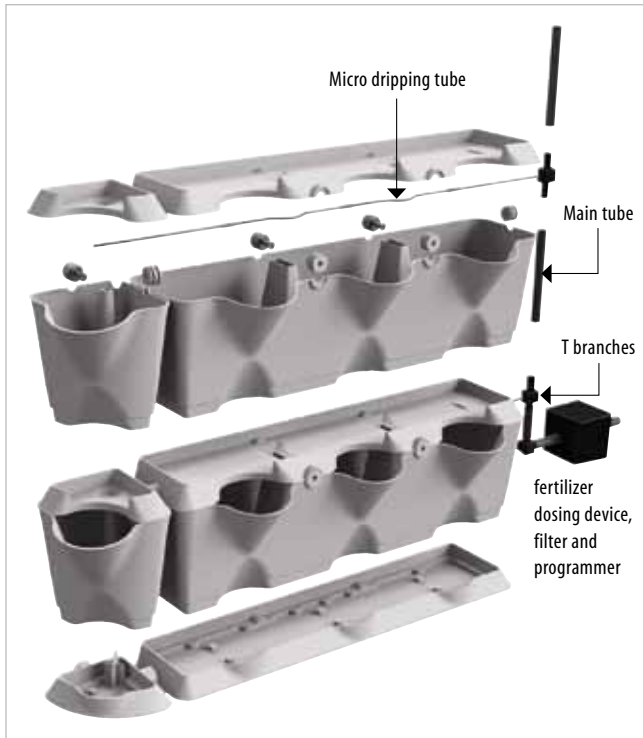
Watering system
