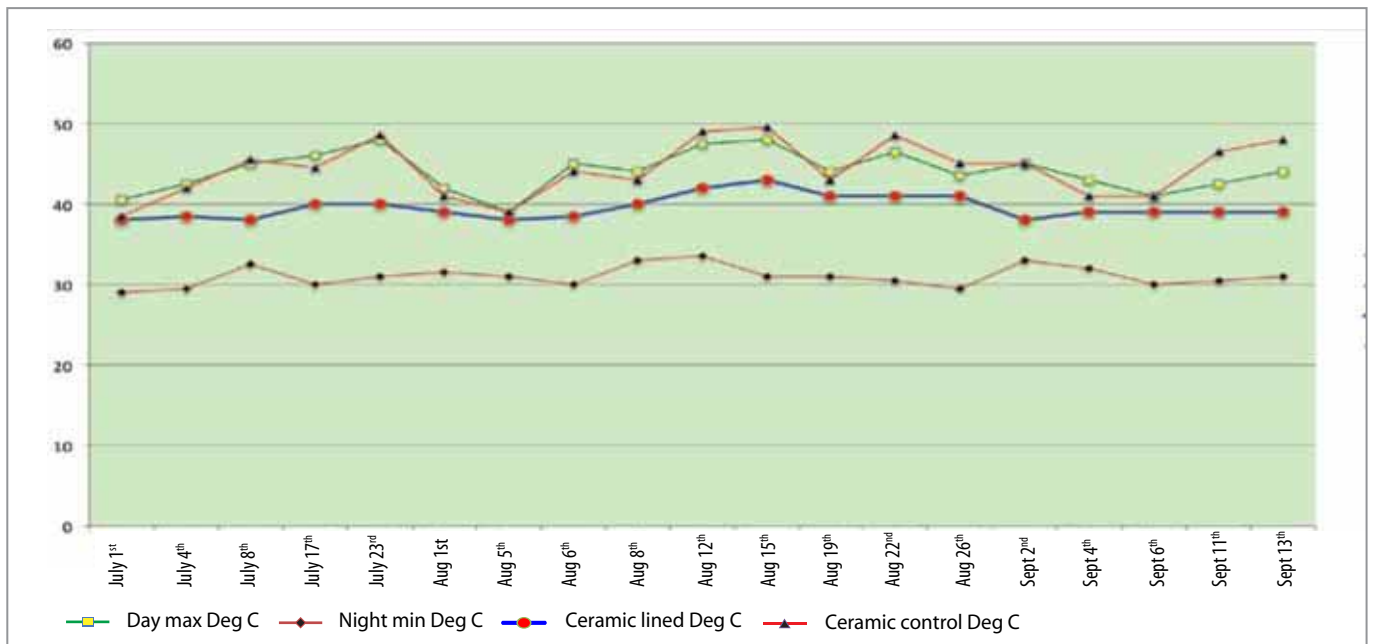
Shows recorded temperatures (ambient - day max. & night min.), compared to ceramic planters with and without a thermal liner
