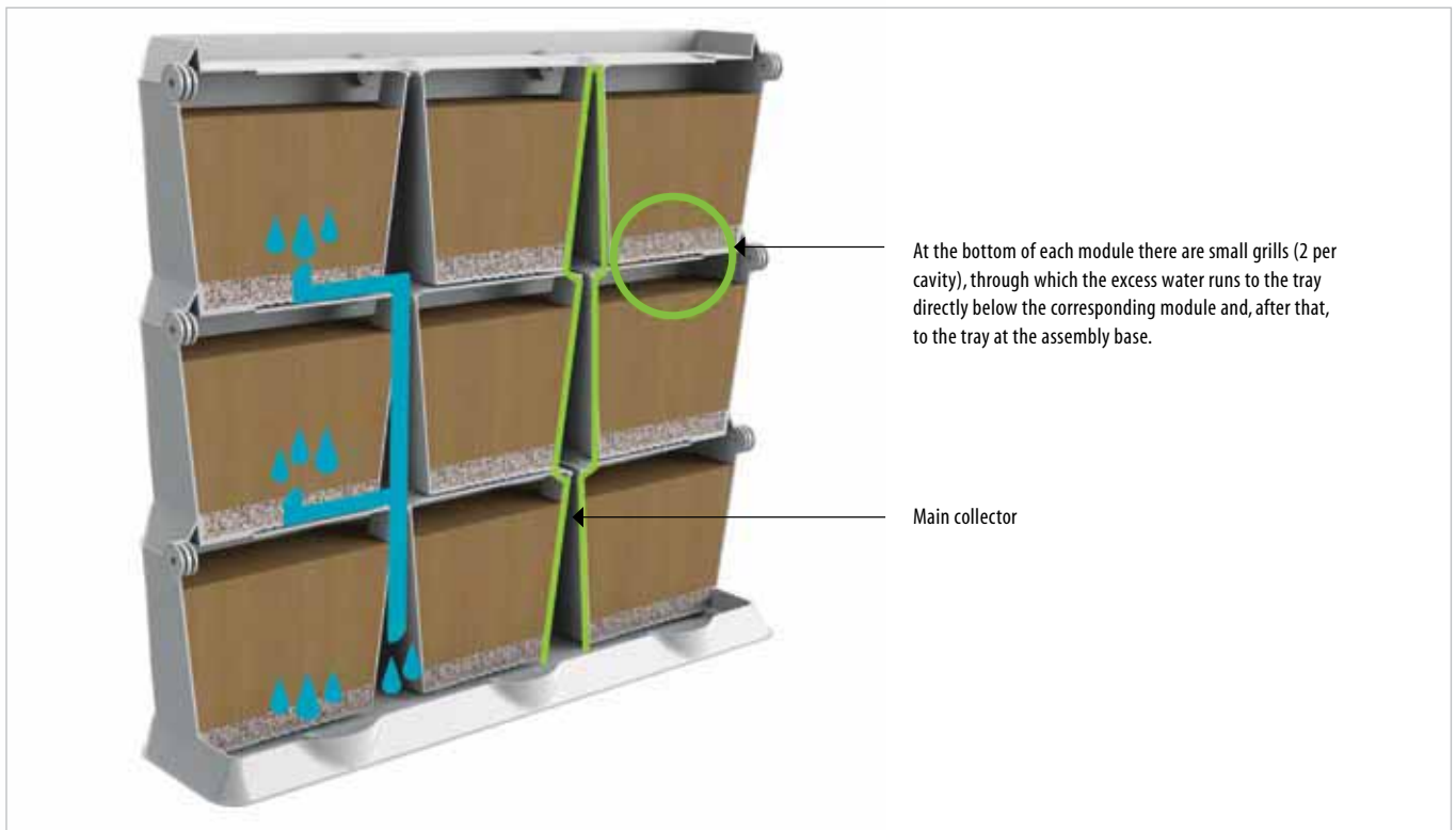
Drainage System
